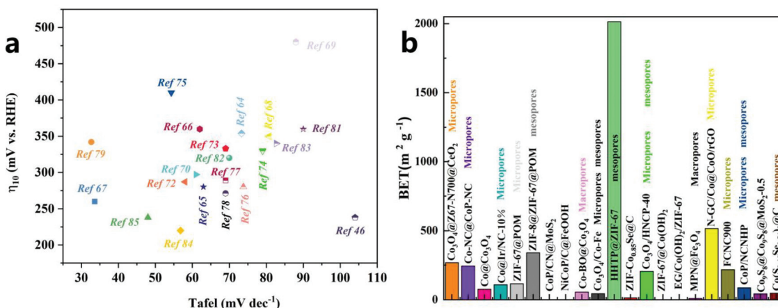
Fig. 6 (a) OER activity comparison graph showing the Tafel slope at an overpotential of 10 mA cm -2 for different catalysts. (b) Comparison of BET/BJH results for different catalysts.
