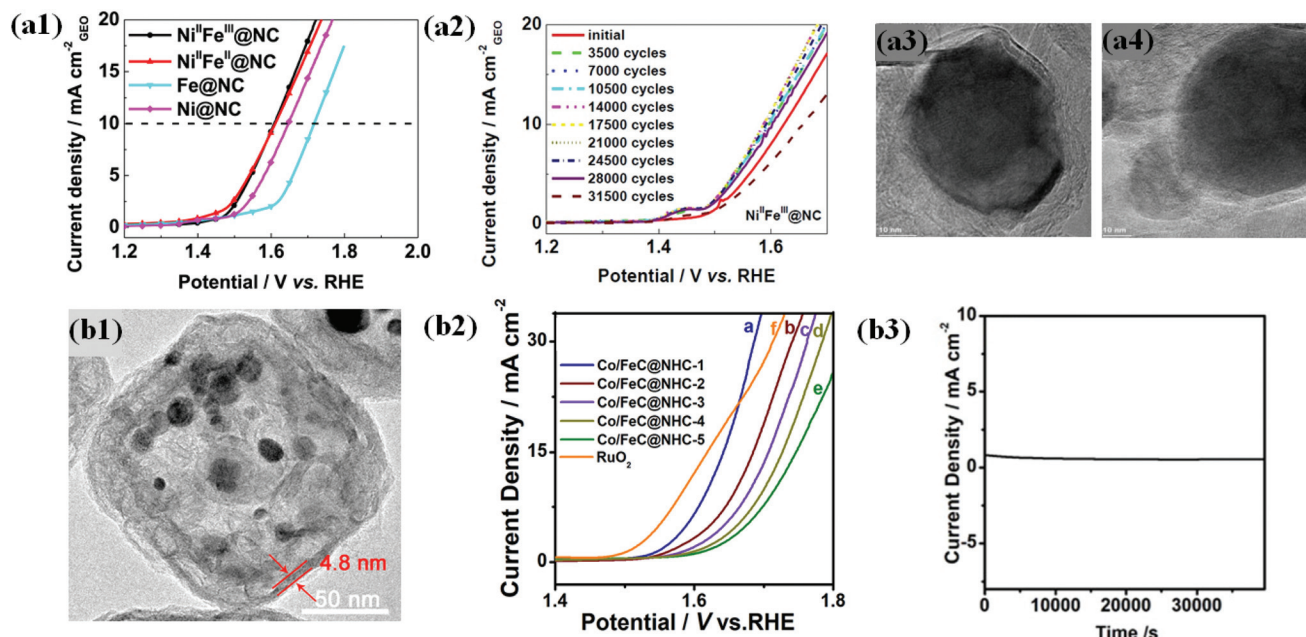
Fig. 9 (a1) LSV curves ( 10 \text{ mV s}^{-1} @ 900 rpm) of \text{Ni}^{\text{II}}\text{Fe}^{\text{III}}@\text{NC} , \text{Ni}^{\text{II}}\text{Fe}^{\text{II}}@\text{NC} , \text{Fe}_4[\text{Fe}^{\text{II}}(\text{CN})_6]_3 derived \text{Fe}@\text{NC} and \text{Ni}^{\text{II}}[\text{Ni}^{\text{II}}(\text{CN})_4] derived \text{Ni}@\text{NC} catalysts in oxygen-saturated 0.1 M KOH solutions. (a2) LSV curves of \text{Ni}^{\text{II}}\text{Fe}^{\text{III}}@\text{NC} after a certain number of ADT cycles between 1.2 and 1.9 V at 500 \text{ mV s}^{-1} . TEM images of (a3) \text{Ni}^{\text{II}}\text{Fe}^{\text{III}}@\text{NC} and (a4) \text{Ni}^{\text{II}}\text{Fe}^{\text{III}}@\text{NC} catalysts after ADT, reproduced with permission from ref. 63, Elsevier copyright 2017. (b1) TEM images of (A) \text{Co/FeC@NHC-1} (b2) OER polarization curves of \text{Co/FeC@NHC-1} , \text{Co/FeC@NHC-2} , \text{Co/FeC@NHC-3} , \text{Co/FeC@NHC-4} , \text{Co/FeC@NHC-5} , and \text{RuO}_2 in 1 M KOH. (b3) Potentiostatic response (current density versus time) under a constant potential of 1.54 V vs. RHE, reproduced with permission from ref. 151, Elsevier copyright 2020.
