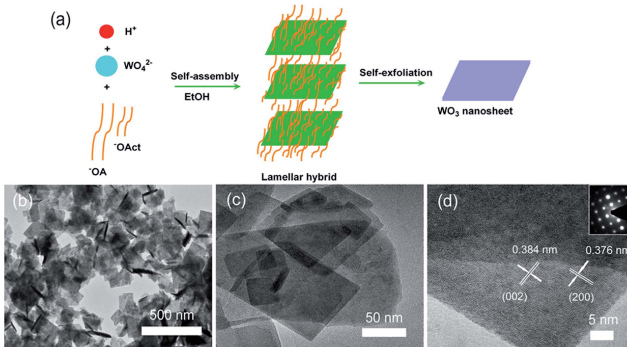
Fig. 3 (a) Schematic of self-assembly. (b–d) SEM, TEM, and HRTEM images of \text{WO}_3 nanosheets produced with a \text{NaOAct}/\text{NaOA} mass ratio of 0.04. Reprinted with permission from ref. 53, copyright 2018, Elsevier.
