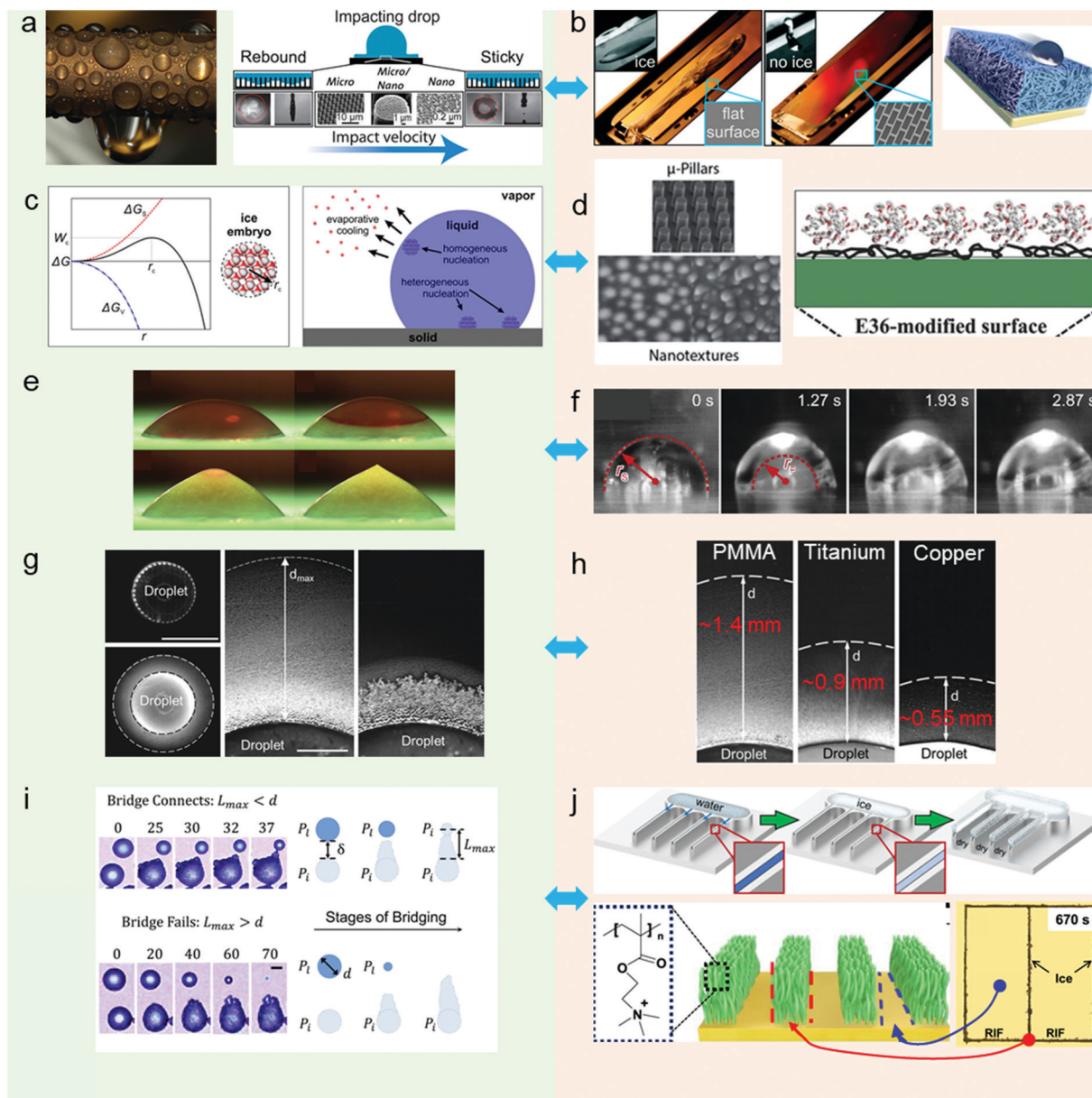
Fig. 1 From the icking process (left, light green background) to anti-icing strategies (right, light orange background). (a) Collection of water via condensation 56 (left; copyright 2013 American Chemical Society) and adhesion of impacting droplets 16 (right; copyright 2014 American Chemical Society). (b) Repelling water droplets by using nanostructured SHS 6 (left, copyright 2010, American Chemical Society) and LIS 30 (right, copyright 2011 Springer Nature). (c) Ice nucleation. 59 Copyright 2015 American Chemical Society. (d) Inhibiting ice nucleation by designing nanostructured surfaces (left, copyright 2014 Royal Society of Chemistry) and supercharged polypeptide surfaces (right, copyright 2016 Wiley-VCH). (e) Ice growth and recrystallization. 61 Copyright 2012 American Institute of Physics. (f) Inwards growth of ice induces spontaneous self-dislodging of droplets. 62 Copyright 2017 National Academy of Sciences. (g) Frost halos. 63 Copyright 2012 National Academy of Sciences. (h) Maximum expanse of PMMA, titanium, and copper under 1.3% humidity. 63 Copyright 2012 National Academy of Sciences. (i) Interoplet ice bridging and dry zones. 64 Copyright 2016 American Chemical Society. (j) Restricting ice propagation by using microscopic ice patterns 65 (top, copyright 2018 American Chemical Society) and grafting patterned polyelectrolyte 66 (bottom, copyright 2020 American Chemical Society).
