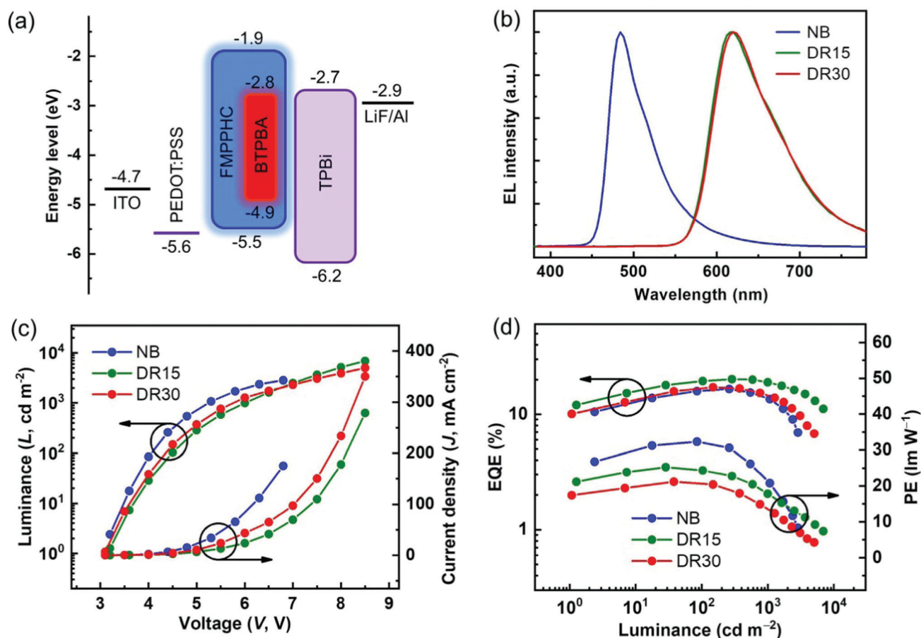
Fig. 3 (a) Proposed energy diagram of the materials used in OLEDs. (b) Normalized EL spectra of devices NB, DR15 and DR30 at the luminance of 1000 cd m -2 . Current density–voltage–luminance ( J – V – L ) curves (c) and power efficiency (PE)–luminance ( L )–external quantum efficiency (EQE) curves (d) of devices NB, DR15 and DR30.
