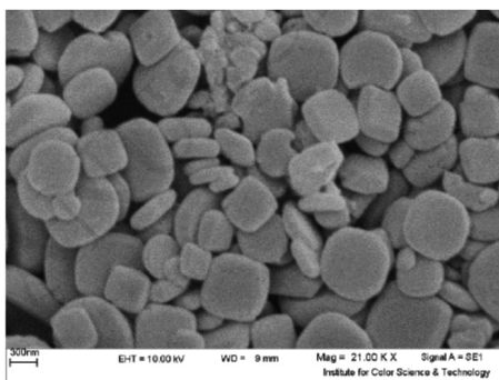
Fig. 13 Morphology of \text{NH}_2 -MIL-125(Ti) with circular plate [Reprinted with permission from ref. 257. Copyright 2018, Elsevier].
