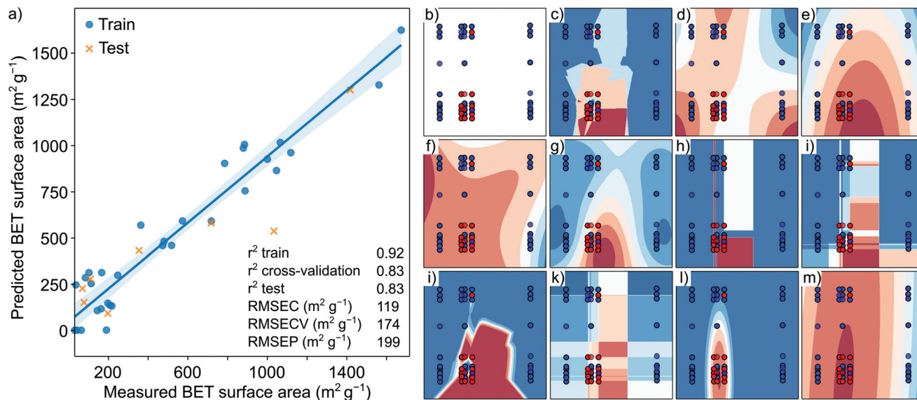
Fig. 5 (a) Visualization of the predicted versus measured BET surface areas (m 2 g -1 ). Visual representation of the binary classification results using different algorithms, where the accuracy score is provided in parenthesis: (b) input data projected on the principal component 1 (x-axis) and principal component 2 (y-axis), (c) k-nearest neighbor algorithm (0.83), (d) sigmoid support vector machine (0.70), (e) radial basis function support vector machine (0.71), (f) polynomial kernel support vector machine (0.71), (g) Gaussian process (0.82), (h) decision-tree algorithm (0.77), (i) random forest algorithm (0.73), (j) artificial neural network (shallow) (0.76), (k) adaptive boosting algorithm (0.79), (l) naive Bayes method (0.87), and (m) quadratic statistical classifier (0.87). The higher the accuracy score, the higher the predictive power of the method.
