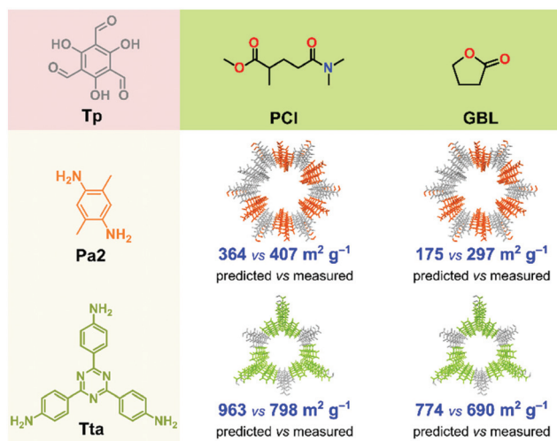
Fig. 6 Comparison of predicted vs. measured SA BET of two COFs synthesized in PCI and GBL solvents.
