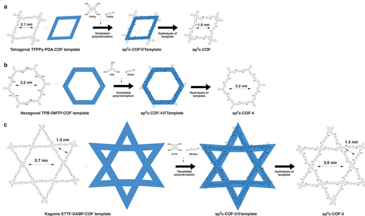
Fig. 17 (a) Topology-templated synthesis of tetragonal sp^2c -COF using the imine-linked TFFPy-PDA-COF as the template. (b) Topology-templated synthesis of hexagonal sp^2 -COF-4 using the imine-linked TPB-DMTP-COF as the template. (c) Topology-templated synthesis of kagome sp^2 -COF-5 using the imine-linked ETTF-DABP-COF as the template. Adapted with permission from ref. 26, Copyright 2020 Wiley-VCH.
