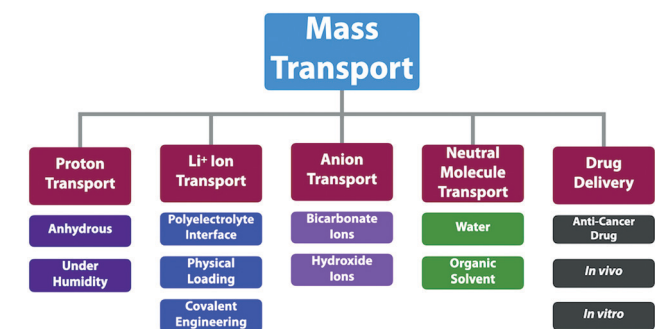
Scheme 10 Strategies for designing COFs to promote mass transport.
