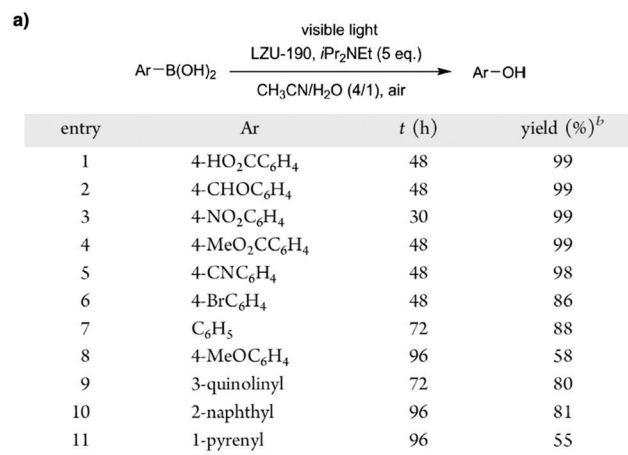
a Conditions: Arylboronic acid (0.2 mmol), LZU-190 (21.2 mg, 0.015 mmol), CH 3 CN (1.6 mL), H 2 O (0.4 mL), iPr 2 NET (5.0 equiv), irradiation with 20 W white LEDs. b Yields of the isolated products.
