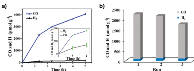
Fig. 95 (a) Photocatalytic evolutions of CO and \text{H}_2 by Ni-TpBpy under 1 and 0.1 atm (diluted with Ar, inset) and (b) stability tests of Ni-TpBpy for selective photoreduction of \text{CO}_2 . Adapted with permission from ref. 177, Copyright 2019 ACS.
