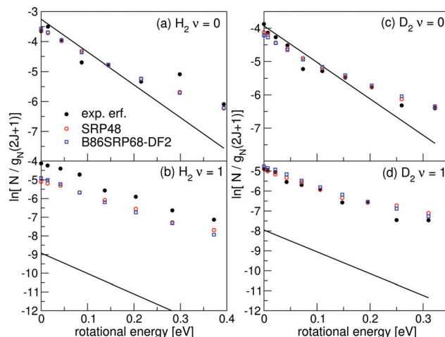
Fig. 17 Rovibrational state populations of H_2 and D_2 desorbing from Au(111) are shown versus the rotational energy. Experimental results are shown in black, 70 theoretical results are shown in red for the SRP48 DF 142 and in blue for the B86SRP68-DF2 DF. The straight lines represent Boltzmann distributions for the surface temperature of the experiment.
