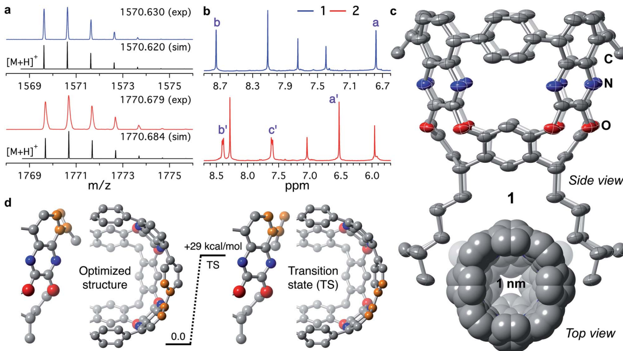
Fig. 1 (a) Experimental MALDI-TOF MS molecular ion peaks of 1 (blue trace) and 2 (red trace). Black traces represent the simulated [M + H]^+ isotopic distributions. (b) ^1\text{H} NMR of (top) 1 and (bottom) 2 in \text{CD}_2\text{Cl}_2 at 20^\circ\text{C} . Proton labels according to Scheme 1. (c) Molecular crystal structure of 1 obtained at 150\text{ K} . Thermal ellipsoids are set at 50\% probability level. The C, N, and O atoms are coloured grey, blue, and red, respectively. The H atoms are omitted for clarity. Bottom: top view of the sphere packing model (van der Waals radii) of 1 . (d) DFT calculated barrier for ring flipping. Rotation of the phenyl moiety was followed by tracking the dihedral angle between the highlighted carbon atoms in orange.
