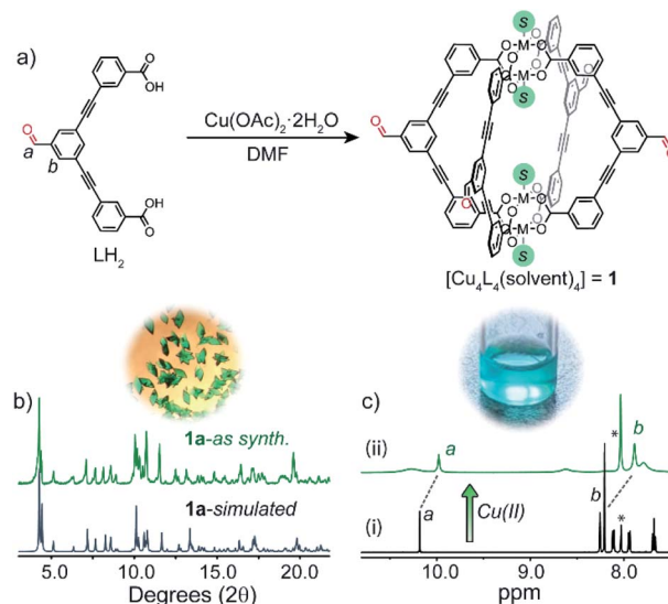
Fig. 2 (a) A scheme showing the self-assembly of 1 in solution from \text{LH}_2 and \text{Cu}(\text{OAc})_2 \cdot 2\text{H}_2\text{O} ( \text{S} = \text{solvent} ); (b) simulated and experimental PXRD patterns of phase 1a ; (c) ^1\text{H} NMR spectrum (500 MHz/ \text{DMF-d}_7 , 25 °C): (i) \text{LH}_2 , (ii) \text{LH}_2 + \text{Cu}(\text{OAc})_2 (* indicates solvent peak). ‡ Above (b) and (c) are photos of crystals of 1a (left) and a DMF solution of 1 (right).
