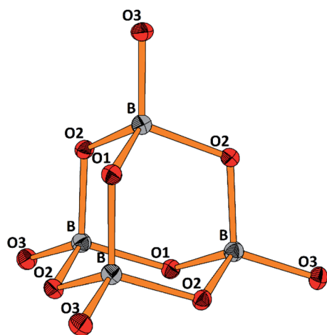
Fig. 5 Perspective representation of the \text{B}_4\text{O}_{10}^{8-} anion. Color code: B (grey), O (red), displacement ellipsoids drawn at the 50% probability level. For the labeling scheme c.f. Tables S2 and S3. †
