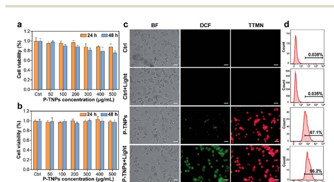
Fig. 4 The cytotoxicity of P-TNPs against (a) 4T1 cells and (b) DC2.4 cells after incubation for 24 h or 48 h. (c) Intracellular ROS generation of P-TNPs against 4T1 cells upon white light irradiation (2000 lm) for 3 min. Emission: BF (bright field), green from DCF, red from the AIE dye (TTMN). Scale bar: 20 \mu\text{m} . (d) Flow cytometry analysis of DCF fluorescence intensity in the corresponding groups.
