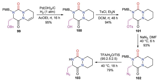
Scheme 37 Hydroxyl substitution with an azide at position 5 of an aza-DKP.
