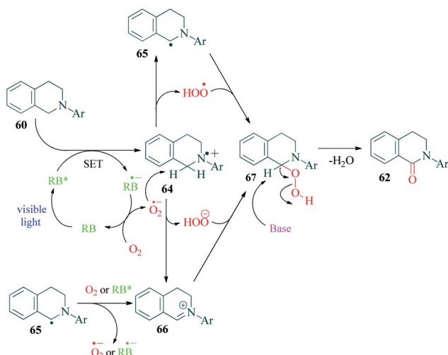
Scheme 18 Rose Bengal catalyzed C–H oxidation of tryptoline and tetrahydroisoquinoline substrates.
