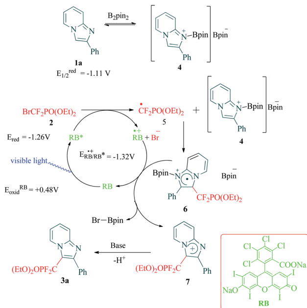
Scheme 2 Rose Bengal catalyzed \text{C}(\text{sp}^2)\text{-H} difluoromethylene-phosphonation of imidazopyridines.
