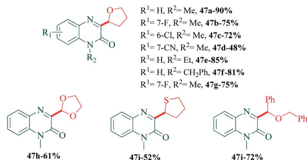
Scheme 13 Visible light promoted 3-oxyalkylation of quinoxalin-2(1H)-ones.
