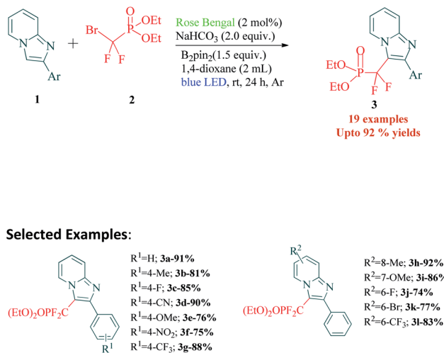
Scheme 1 Visible light promoted difluoromethylene-phosphonation of imidazoheterocycles.
