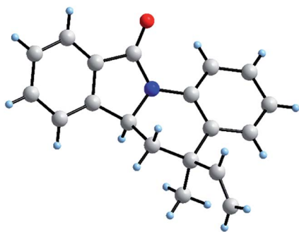
Fig. 4 Stick-ball model of 6a asymmetric unit from monocrystal X-ray diffraction (see ESI†).
