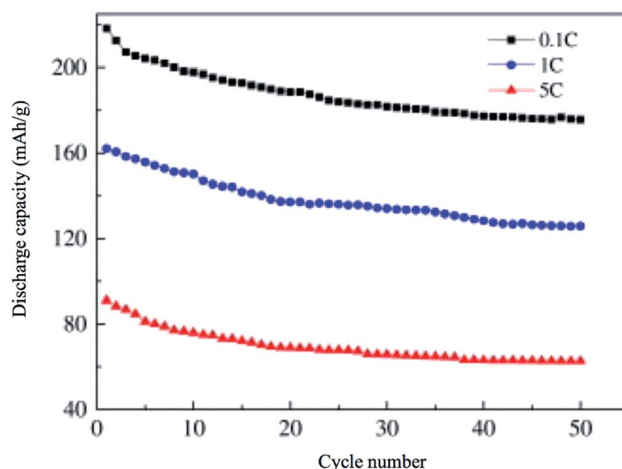
Fig. 17 Cyclic performance of nano \text{C/Li}_2\text{MnSiO}_4 synthesized by ionothermal method, the material is tested in the potential range of 2.5–4.5 V. 153
