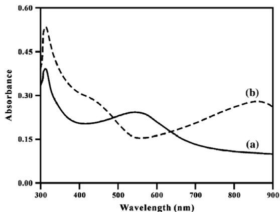
Fig. 14 Electronic spectrum of undoped (a) and doped (b) poly[bis(2-aminophenoxy)disulfide] in DMF. Reproduced with permission from ref. 101.
