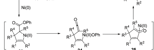
Scheme 18 Ni-Catalyzed reductive [3 + 2] cycloaddition of alkynes with \alpha,\beta -unsaturated carbonyl compounds.
