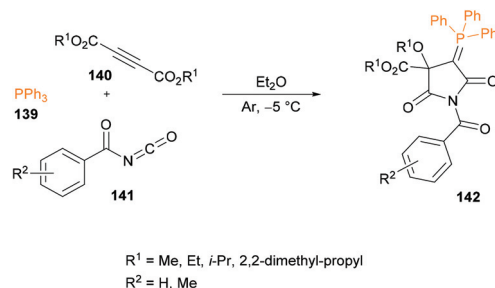
Scheme 32 Three-component synthesis of highly functionalized triphenylphosphoranylidene succinimides.
