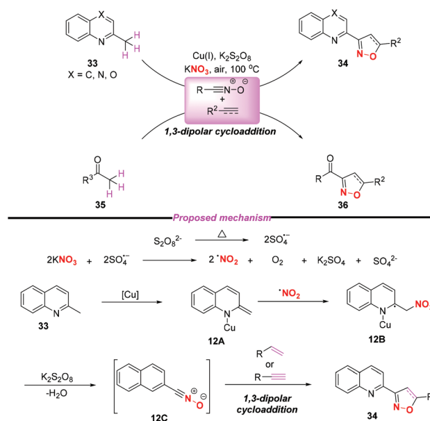
Scheme 12 Copper-catalyzed \text{sp}^3 C–H bond oxidative functionalization of alkylazaarenes.
