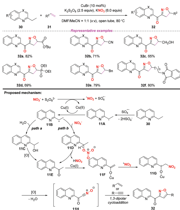
Scheme 11 Copper-catalyzed selective cascade \text{sp}^3 C–H bond oxidative functionalization of 2-ethylazaarenes.
