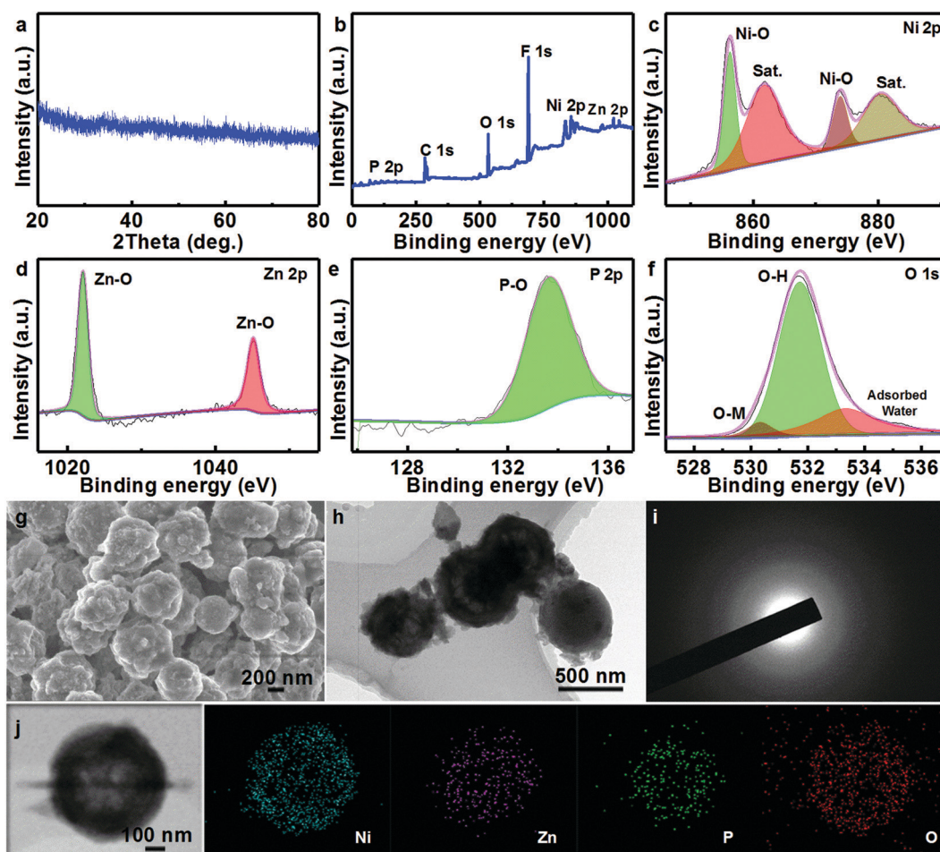
Fig. 4 Microstructure characterizations of the yolk-shell NNP HMSs after long-term durability test. (a) XRD pattern; XPS spectra for (b) survey pattern, (c) Ni 2p, (d) Zn 2p, (e) P 2p and (f) O 1s; (g) FESEM image; (h) TEM image; (i) SAED pattern; (j) STEM and corresponding elemental Ni, Zn, P and O mapping images.
