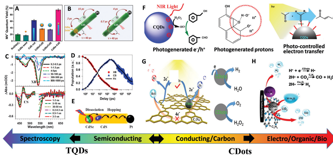
Fig. 10 Catalytic applications of TQDs and CDots. (A) Photocatalytic activity of various TQD structures with different charge separation arrangements for the quantum yield of photogenerated MV^{+\bullet} (methyl viologen) radicals. Reprinted with permission from ref. 234, Copyright 2012, American Chemical Society. (B) Photogenerated charge carrier decay dynamics in the CdSe@CdS–Pt dot@rod (left) and CdS/Pt nanorods (right) obtained from transient absorption measurements. Reprinted with permission from ref. 235, Copyright 2015, American Chemical Society. (C) Representative transient absorption spectra of CdSe@CdS–Pt nanorods upon excitation of the CdSe core. (D) Kinetics of exciton bleach (XB) and charge separated states (CS) from 1 to 3000 ns. Reprinted with permission from ref. 236, Copyright 2014, American Chemical Society. (E) Plausible mechanism for the long-range charge transfer in CdSe@CdS–Pt NRs, including electron/hole dissociation and random electron hopping. Reprinted with permission from ref. 237, Copyright 2016, The Royal Society of Chemistry. (F) Schematic representation of versatile functions of CDots for catalysis: photogenerated e^-/h^+ , photogenerated protons and photo-controlled electron transfer. (G) Schematic mechanism of the two-step 2e^- - 2e^- photocatalytic water splitting process in the g- C_3N_4 /CDots system. Adapted with permission from ref. 238, Copyright 2015, the American Association for the Advancement of Science. (H) Schematic three-component electrocatalyst design for syngas production by coupling the HER catalyst ( Co_3O_4 ) with the CO_2 reduction catalyst (CDots- C_3N_4 ), employing the adsorption capacity of CDots for CO_2 molecules and protons. Reprinted with permission from ref. 239, Copyright 2017, Nature Publishing Group.
