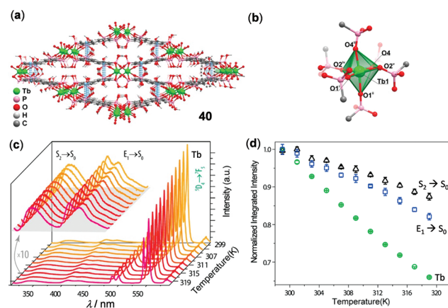
Fig. 32 (a) Crystal packing network and (b) Tb(III) octahedral coordination environment of Tb MOF 40 . (c) Temperature-dependent solid-state emission spectral change of 40 in the range of 299–319 K ( \lambda_{\text{ex}} = 300 nm). (d) Temperature dependence of integrated intensities of different emissions. Reprinted with permission from ref. 142. Copyright 2017 American Chemical Society.
