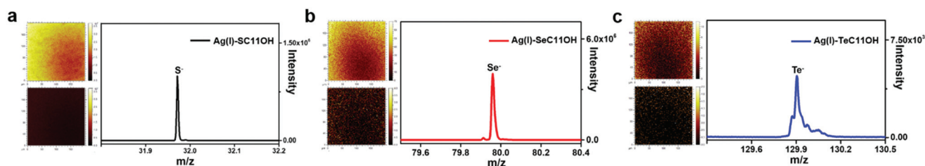
Fig. 2 TOF-SIMS results of silver substrates modified with HOC11X ( X = S, Se, \text{ and } Te ) in the negative mode. (a) Left: TOF-SIMS mapping pictures of S^- ions on the silver substrate before (bottom) and after (top) being modified with HOC11S, in which the yellow the color, the higher the content of S^- ; Right: The peak at 32.0 represented one of the isotopes of sulfur. (b) The results of the silver substrate modified with HOC11Se and the peak at 80.0 represented one of the isotopes of selenium. (c) The results of the silver substrate modified with HOC11Te and the peak at 129.9 represented one of the isotopes of tellurium. All the above mapping pictures showed a little bit non-uniform distribution of chalcogenide anions, which was caused by the error of the instrument itself.
