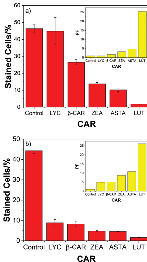
Fig. 3 (a) Dead cell count compared for 5 carotenoids against the control at 100% oxygen. (b) Dead cell count compared for 5 carotenoids against the control in air; insets shows the PFs under the same conditions.
