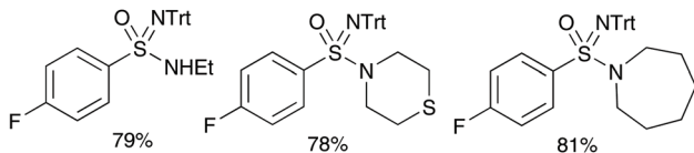
Scheme 17 (a) Bolm's synthesis of sulfonimides 69 from N -tritylsulfonamide 67 , heteroaryl diazonium salts 68 and 1-hydroxybenzotriazole; (b) application to access sulfonimidamides 71 from sulfonimides 70 .
