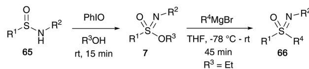
Selected examples of sulfonimides accessed
