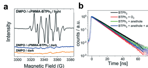
Fig. 3 (a) EPR spectra of DMPO–O 2 •− adducts with cPMMA-BTPH 2 as the photocatalyst in darkness and under blue light irradiation ( \lambda = 460 nm, 1.2 \text{ W cm}^{-2} ). (b) Time-resolved photoluminescence spectra of BTPH 2 under N 2 (black), under O 2 (red), and with trans -anethole under N 2 (green) and in air (blue) with 20 \text{ mg mL}^{-1} of BTPH 2 and 2 \text{ mM} trans -anethole in acetonitrile.
