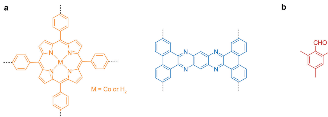
Fig. 32 Useful molecular scaffolds for bottom-up synthesis of COFenes. (a) Backbone functionalities. (b) Inhibitor for crystal growth.
