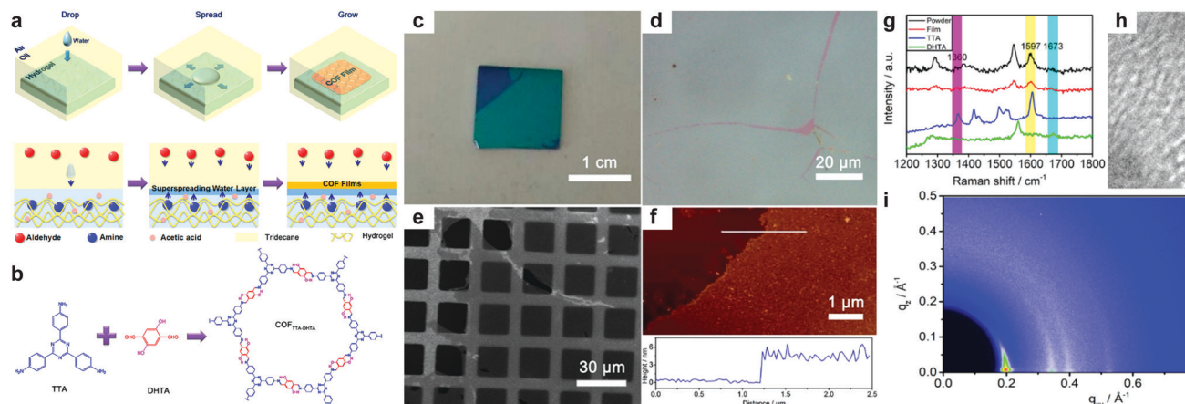
Fig. 35 (a) Scheme of triphase confined synthesis of COFenes. (b) Synthesis of COF TTA-DHTA . (c) Photo image of the COF TTA-DHTA film on a silica wafer. (d) Optical microscopic image of the COF TTA-DHTA film. (e) SEM image of the COF TTA-DHTA film on TEM grids. (f) AFM height image of the COF TTA-DHTA film on a silica wafer. (g) Raman spectra of the COF TTA-DHTA film and powder, and the monomers. (h) TEM images of the COF TTA-DHTA film. Inset: SAED pattern of the films. (i) GIWAXS of the COF TTA-DHTA thin film. Reproduced with permission from ref. 25. Copyright 2018. American Chemical Society.
