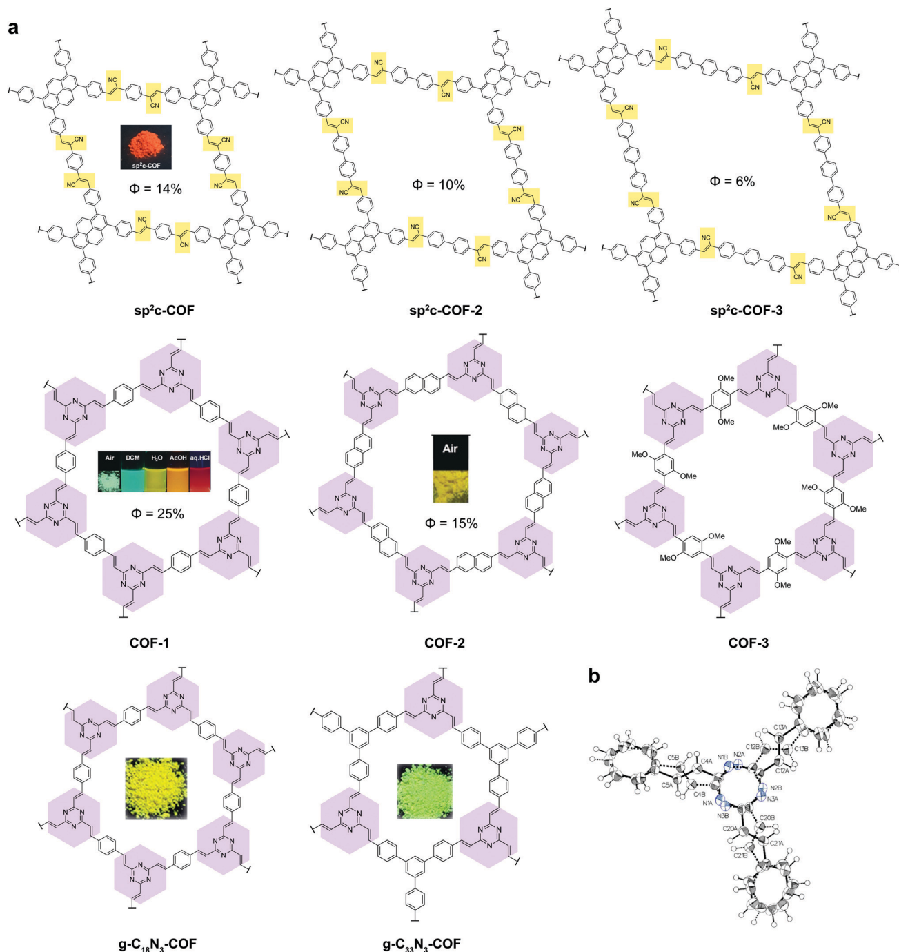
Fig. 6 Solid-state fluorescent 2D COFs based on C=C linkages. (a) Structures of the 2D COFs. (b) Single-crystal structure of the model compound tristyriltriiazine.
