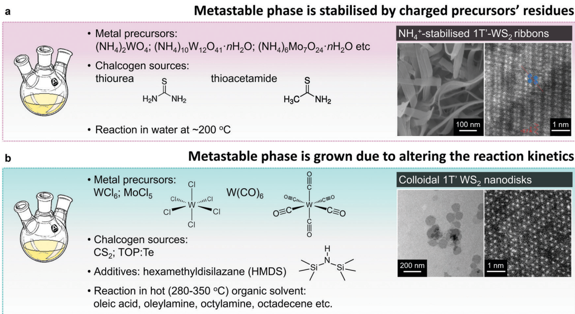
Fig. 6 Direct solution-phase growth of the 1T' polymorphs. (a) Hydro-/solvothoermal reactions between the ammonium containing precursors produce the metastable 1T' phase stabilised by precursors' residues. (b) Colloidal synthesis of the metastable 1T' phase achieved due to the fine control over the reaction kinetics. Figures in panels (a) and (b) are adapted with permission from ref. 82, copyright 2015, John Wiley & Sons, and ref. 80, copyright 2014, American Chemical Society.
