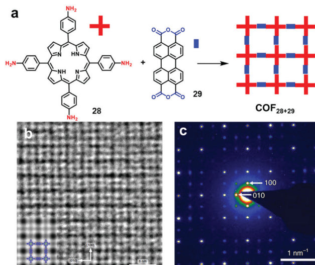
Fig. 21 (a) Schematic illustration of the synthesis of \text{COF}_{28+29} ; (b) AC-HRTEM image of \text{COF}_{28+29} . Inset: A simulated image of \text{COF}_{28+29} along the [001] projection with the structure model overlaid; (c) SAED pattern. The arrows indicate the 100 and 010 reflections at 0.33 \text{ nm}^{-1} . Reproduced with permission from ref. 34 Copyright 2019, Springer Nature.
