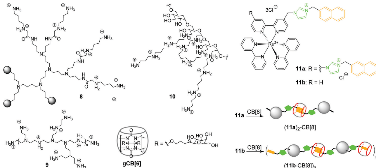
Scheme 2 Structures of cationic dendrimers 8–10 , the galactosylated cucurbit[6]uril ( gCB[6] ), bis-naphthalene-derivatized \text{Ru}(\text{bpy})_3 guests 11a and 11b and their supramolecular assembly in CB[8] cavity.
