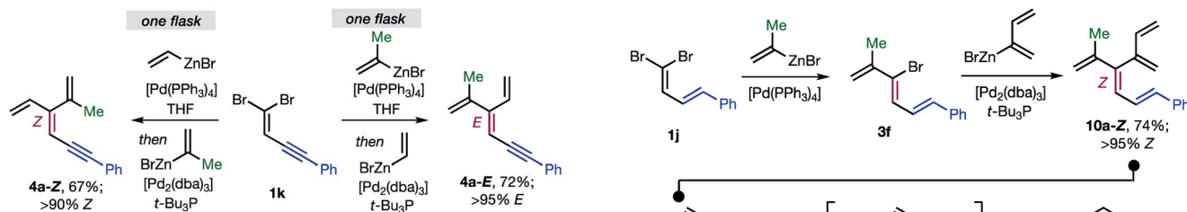
Scheme 1 One flask stereoselective syntheses of E - and Z -diastereomers of dendralene 4a from 1,1-dibromide 1k .
