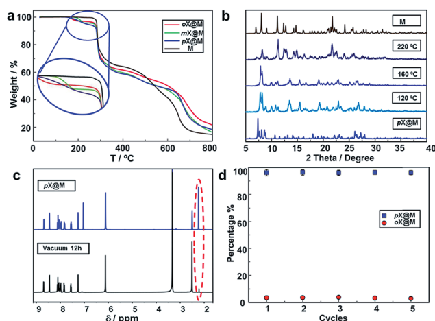
Fig. 4 Recyclability of M . (a) The TGA profiles for M , oX @ M , mX @ M , pX @ M . Loss of weight: pX @ M > mX @ M > oX @ M . (b) VT-XRD experiments for pX @ M . With the temperature increasing, the pattern of PXRD transformed from pX @ M into M . (c) The 1 H NMR spectra of pX @ M and the sample after vacuum drying. (d) Relative uptake of pX and oX in M after M is recycled for 5 times.
