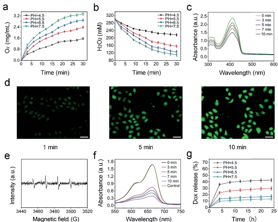
Fig. 4 Production of O 2 (a) and decomposition of H 2 O 2 (b) catalyzed by UCNP@mCeO x aqueous solution in 30 min. NPs were observed under 980 nm laser irradiation. The absorbance of DPBF solutions with UCNP@mCeO x at different time periods under 980 nm laser irradiation (0.72 W cm -2 ) (c). The CLSM images of HeLa cells with oxidized DCF fluorescence at different illumination times (d). ESR spectra for detection of hydroxyl radicals versus magnetic field (e). UV-vis absorption spectra of MB solution with UCNP@mCeO x at different light times (f). Release rate of DOX in PBS under different pH conditions as a function of the release time (g).
