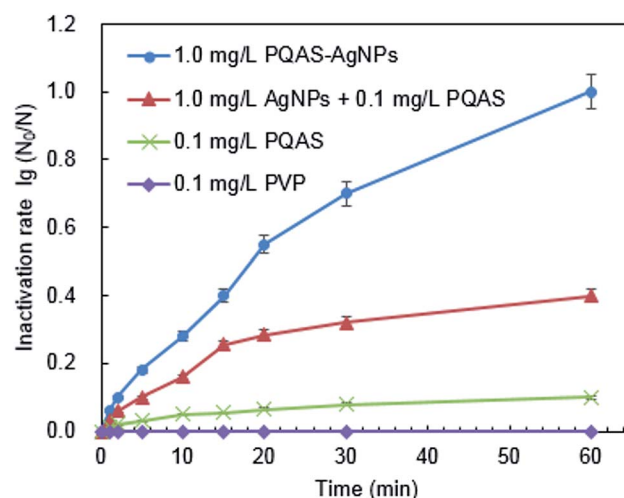
Fig. 3 The role of PQAS and AgNPs in the antibacterial activity of PQAS-AgNPs. Reaction conditions: reaction time = 60 min, pH = 7.1, T = 25 °C, initial concentration of B. subtilis : 10 6 CFU mL -1 .
