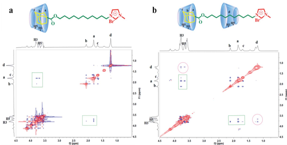
Fig. 5 ^1\text{H} - ^1\text{H} 2D ROESY spectra of 10 mM AD- \text{C}_{11}\text{im}@1\beta\text{-CD} (a) and 10 mM AD- \text{C}_{11}\text{im}@2\beta\text{-CD} (b).
