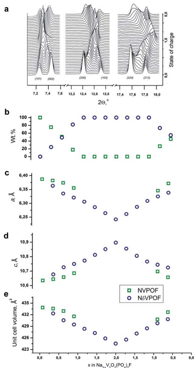
Fig. 9 Results of operando SXPED experiments on \text{Na}_3\text{V}_2\text{O}_2(\text{PO}_4)_2\text{F} : (a) evolution of the selected regions of the SXPED patterns; (b) mass fraction; and (c–e) unit cell parameters of sodiated (NVPOF) and desodiated ( \text{N}_\delta\text{VPOF} ) phases.
