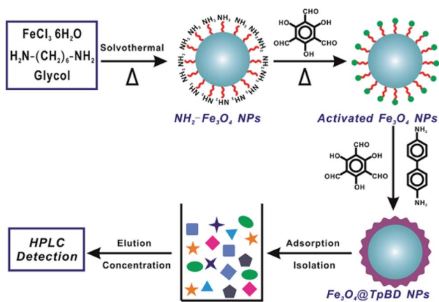
Fig. 1 Schematic illustration of magnetic core-shell covalent organic frameworks as efficient solid-phase extraction adsorbents for determination of sulfonamides residues.
