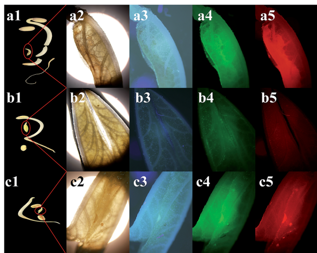
Fig. 8 Images of the mung bean sprouts under (a1, b1, and c1) daylight, (a2, b2, and c2) bright field, (a3, b3, and c3) UV (405 nm), (a4, b4, and c4) blue (488 nm) and (a5, b5, and c5) green light (546 nm). (a, b and c) Show the images of the mung bean sprouts incubated with the N-CD solution, the N-CD + Cr(vi) solution and N-CD + Cr(vi) + AA solution, respectively. The concentrations of the N-CDs, Cr(vi) and AA solution were 0.1 \text{ mg mL}^{-1} , 50 \mu\text{M} , and 100 \mu\text{M} , respectively.
