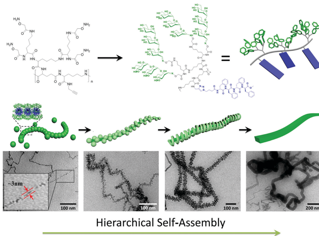
Fig. 24 Hierarchical self-assembly of alternating amphiphilic glycopolymer brushes with pendants of high-mannose glycodendron and oligo-phenylalanine. Reprinted with permission from ref. 176. Copyright 2016, American Chemical Society.
