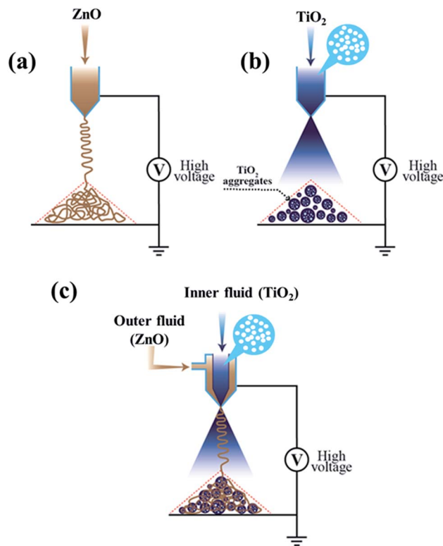
Fig. 1 Schematic diagram of (a) e-spray process for ZnO nanofiber preparation, (b) formation of TiO 2 nanobeads using e-spraying, and (c) co-axial e-spray process for the formation of hybrid films.
