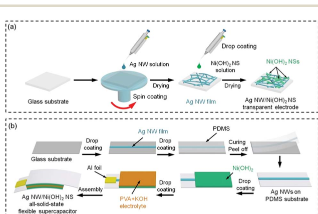
Scheme 1 Schematic of the fabrication of (a) the Ag NW/ \text{Ni}(\text{OH})_2 NS TE and (b) the all-solid-state flexible supercapacitor.
