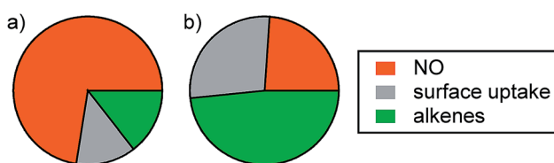
Fig. 7 Relative contribution of the three sinks to O_3 loss in the environmental chamber under (a) post-cooking and (b) background conditions. The contribution of alkenes is determined based on the O_3 loss that is not accounted for by the other two processes.
