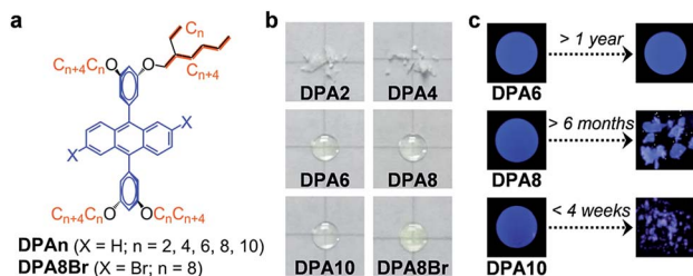
Fig. 1 (a) Chemical structures of DPAn ( n = 2, 4, 6, 8, and 10 ) and DPA8Br. (b) Photographs of freshly synthesized DPAn and DPA8Br in daylight at 20\text{ }^\circ\text{C} , with a drop of fluid or powder of solid on a glass plate. (c) Photographs of DPA6, DPA8, and DPA10 as fresh (left) and after long-term of aging at ambient temperature (right) taken under irradiation of a UV lamp ( 365\text{ nm} ).
