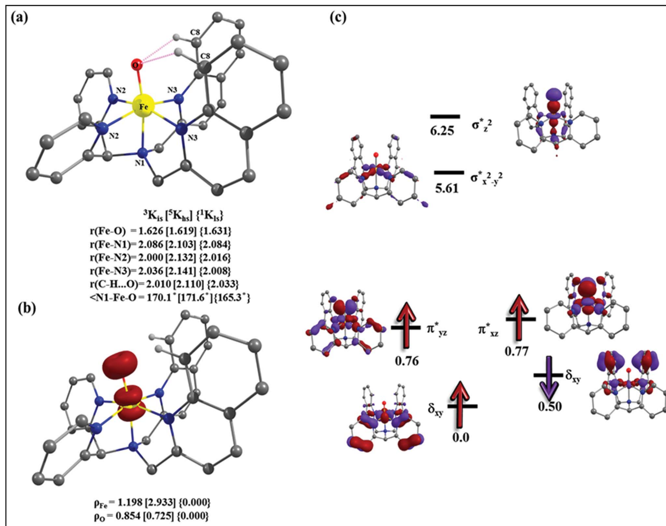
Fig. 9 (a) Important structural parameters and (b) spin densities of B3LYP-D2 optimized structures of [\text{Fe}^{\text{IV}}(2\text{PyN2Q})(\text{O})]^{2+} , and (c) key orbitals of ^3K .
