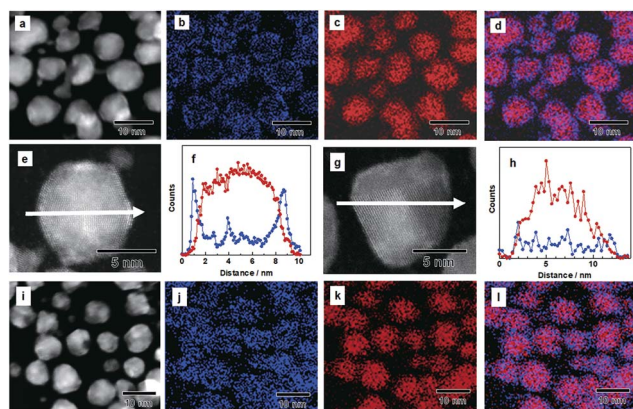
Fig. 1 (a) HAADF-STEM image and EDX maps of (b) Ir and (c) Pd in Pd–Ir NPs before the PHAD. (d) Overlay image of (b) and (c) (blue, Ir; red, Pd). (e) HAADF-STEM image of an as-prepared Pd–Ir NP with a line scan arrow. (f) Line-scanning profiles of Ir (blue) and Pd (red) across the NP. (g) HAADF-STEM image of a Pd–Ir solid-solution NP with a line scan arrow. (h) Line-scanning profiles of Ir (blue) and Pd (red) across the NP. (i) HAADF-STEM image and EDX maps of (j) Ir and (k) Pd in Pd–Ir solid-solution NPs after the PHAD. (l) Overlay image of (j) and (k) (blue, Ir; red, Pd).
