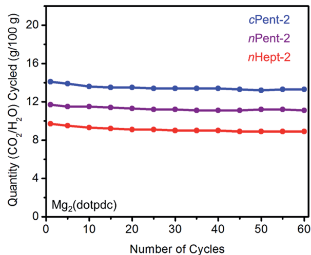
Fig. 10 Cycling stability of 1°,2°-alkylethylenediamine-appended variants of \text{Mg}_2(\text{dotpdc}) in a simulated temperature swing adsorption process. Adsorption conditions: humid 15% \text{CO}_2 in \text{N}_2 , 40 °C, 5 min; desorption conditions: humid \text{CO}_2 , 140 °C, 5 min. Over 60 cycles, the diamine loadings decreased by 10%, 3%, and 3% for cPent-2, nPent-2, and nHept-2, respectively.
