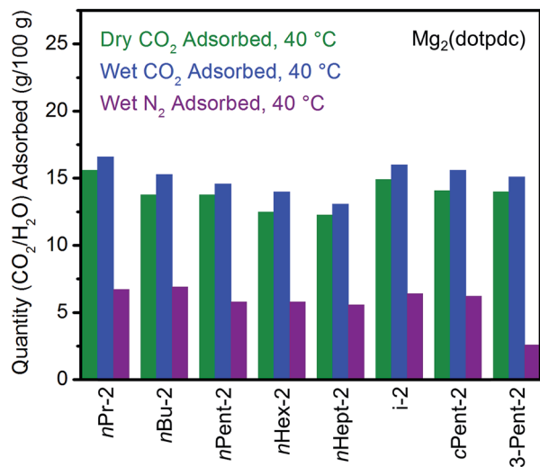
Fig. 9 Summary of the adsorption capacities at 40 °C for a series of 1°,2°-alkylethylenediamine-appended variants of \text{Mg}_2(\text{dotpdc}) under dry \text{CO}_2 (green), humid \text{CO}_2 (blue), and humid \text{N}_2 (purple).
