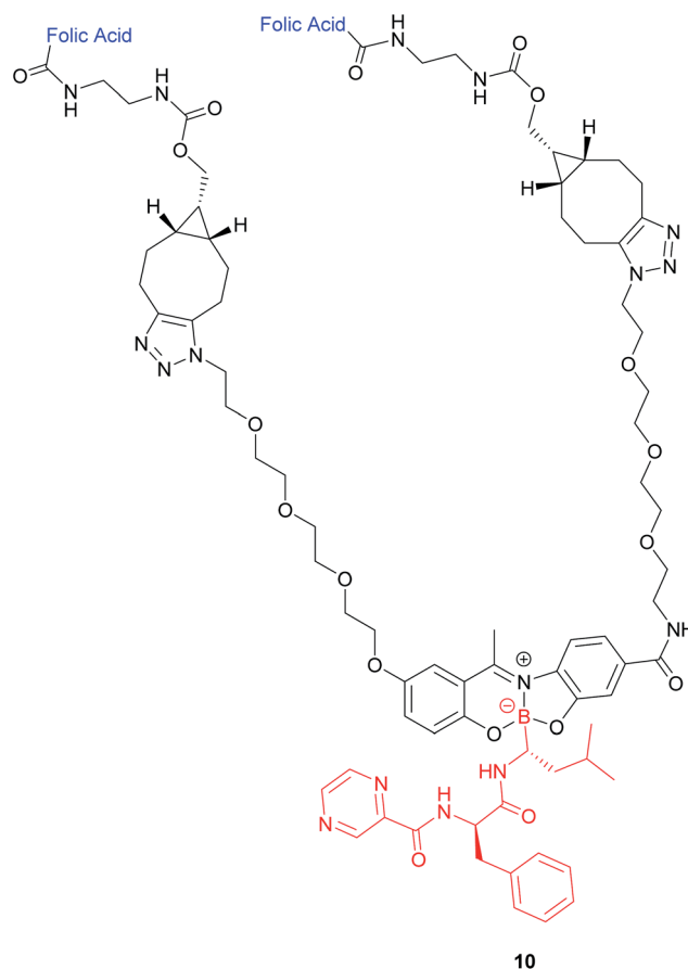
Fig. 8 Structure of the boron complex 10 developed by Gois et al. consisting of (i) a folate acid targeting moiety (blue), (ii) PEG chains and (iii) the cytotoxic agent bortezomib (red). 47
