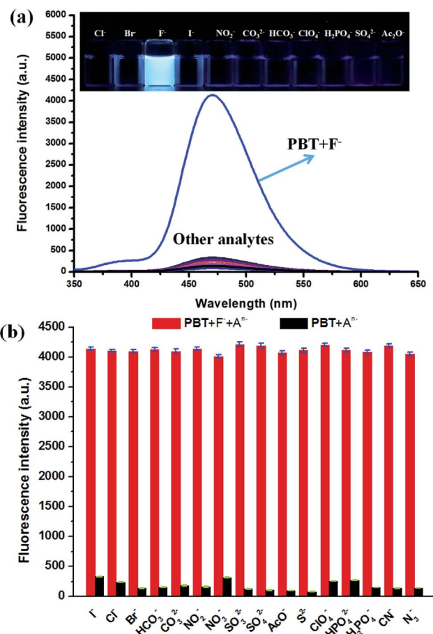
Fig. 6 (a) Fluorescence spectra of PBT in the presence of various anions. [PBT] = 10\ \mu\text{M} , [A^-] = 20\ \mu\text{M} , in a mixture of THF and Tris buffer solution (pH 8.0), (1 : 9, v/v), \lambda_{\text{ex}} = 335\ \text{nm} , \lambda_{\text{em}} = 470\ \text{nm} . Inset: direct observation of fluorescence emission difference of the probe PBT ( 10\ \mu\text{M} ) under UV irradiation (365 nm) in the presence of different anions. Left to right: \text{Cl}^- , \text{Br}^- , \text{I}^- , \text{F}^- , \text{NO}_2^- , \text{CO}_3^{2-} , \text{HCO}_3^- , \text{ClO}_4^- , \text{H}_2\text{PO}_4^- , \text{SO}_4^{2-} and \text{AcO}^- . (b) The selectivity of PBT in the presence of various anions.
